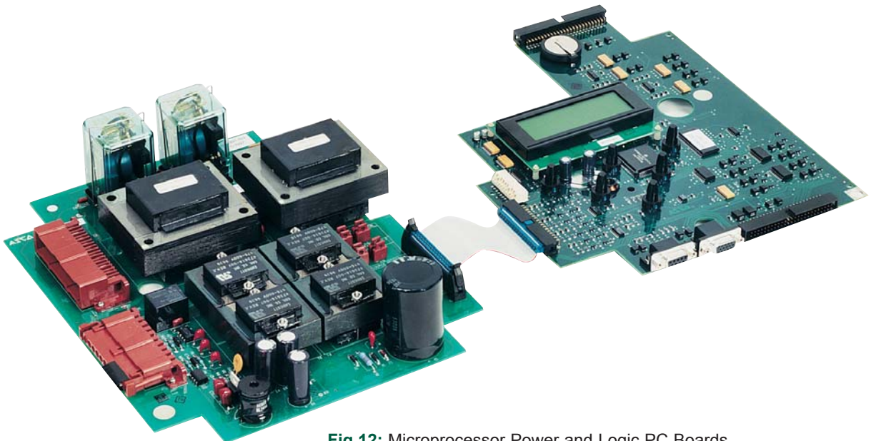
Fig.12: Microprocessor Power and Logic PC Boards.
