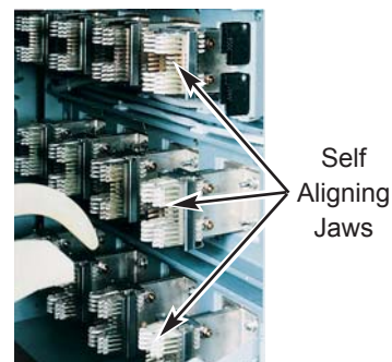
Fig. 7: Bypass-Isolation Transfer Switch self aligning power jaws.
