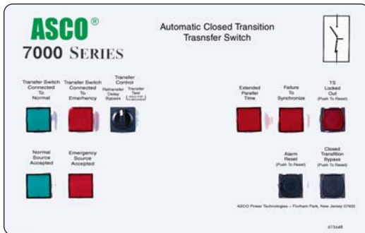
Fig. 14: 7000 Series User Controls and Indicators.
